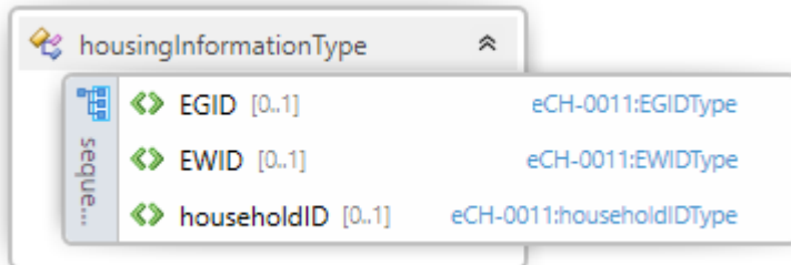
Figure 25: hosingInformationType
