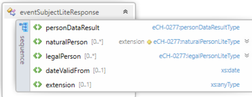
Figure 6: subjectLiteResponse
