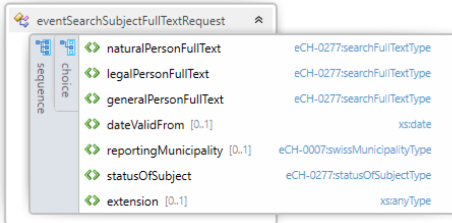
Figure 4: SearchSubjectFullTextRequest
