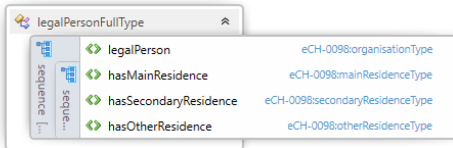
Figure 15: legalPersonFullType
