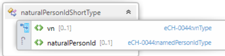
Figure 13: naturalPersonIdShortType
