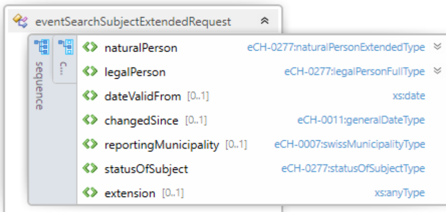
Figure 3: SearchSubjectExtendedRequest
