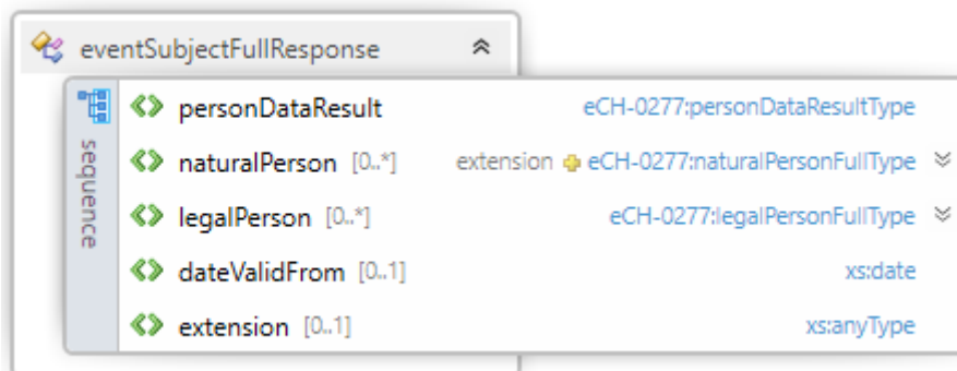
Figure 7: subjectFullResponse
