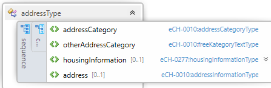
Figure 24: adressType
