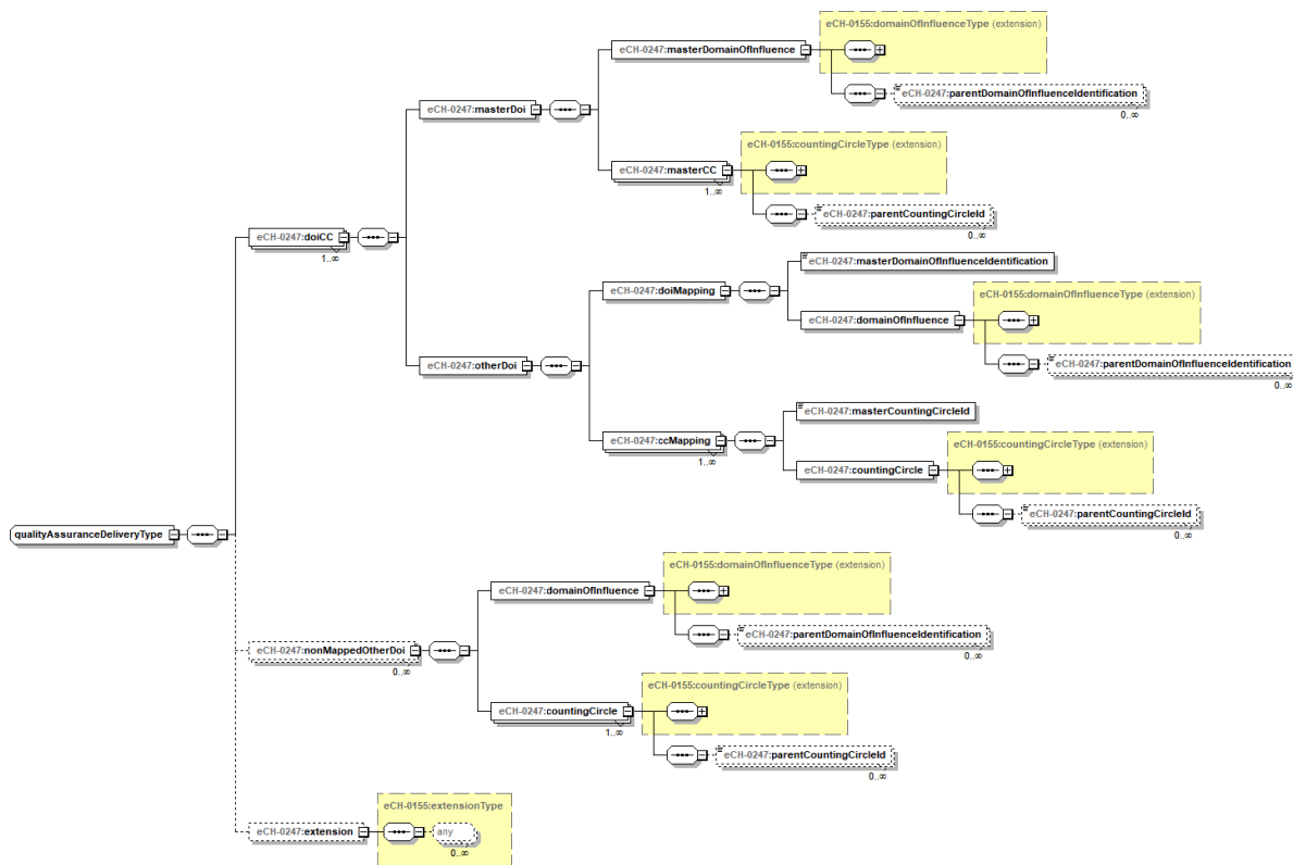
Abbildung 8: qualityAssuranceDelivery
