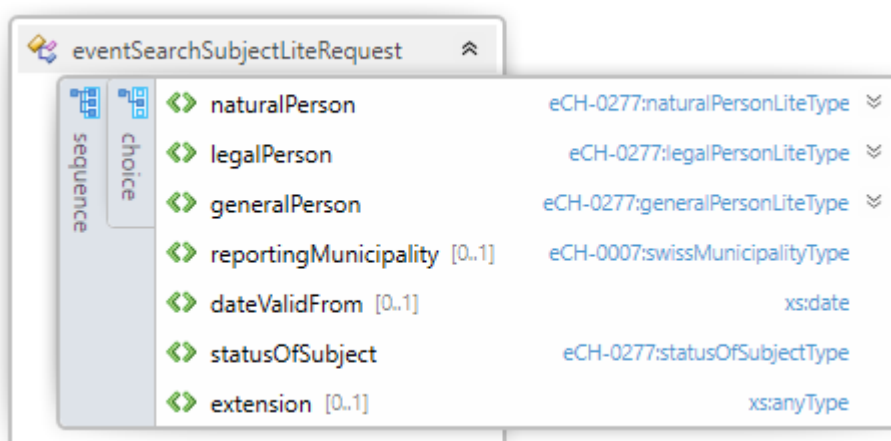
Abbildung 2: SearchSubjectLiteRequest
